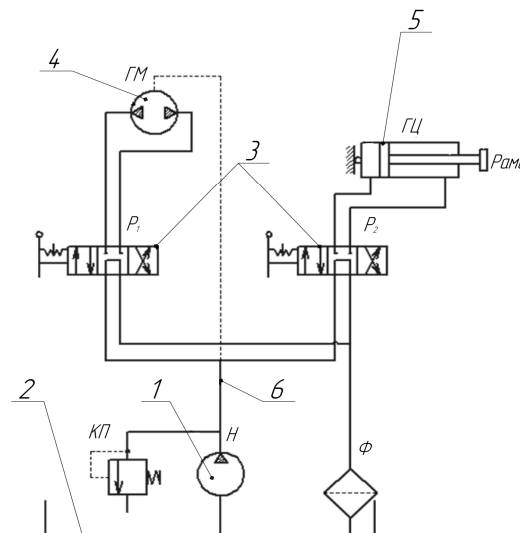
Fig. 3. Schematic diagram of the hydraulic mower unit: 1 – water pump, 2–hydro tank, 3–distributors, 4–hydraulic engine, 5–cylinder, 6–line forcing
