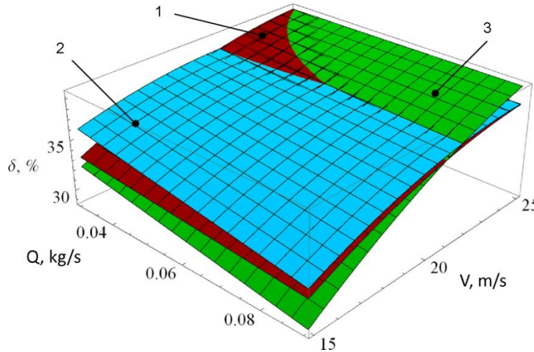
Fig. 7 – The dependence of the distribution coefficient \delta on the seeds supply Q and air flow velocity V 1 – experimental dependence (10); 2 – theoretical dependence (8) with D_{p1} = 6 \text{ mm} ; 3 – theoretical dependence (8) with D_{p2} = 7 \text{ mm}
