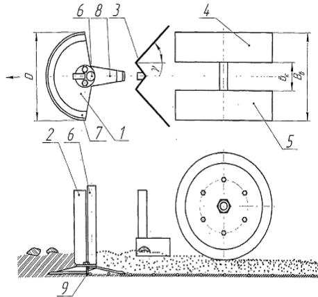
Fig. 11. Scheme of the multipurpose opener group of a row seeder: 1 - a plate opener; 2 - stable; 3 - lump separator - equalizer; 4,5 - the right and left parts of a copying roller; 6 - seminal vesicle; 7 - horizontal lunch; 8 - ending; 9 - knife-shaped device.
