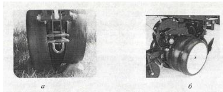
Fig. 8. Location of copying rollers next to the opener: a - copying wheels with a movable suspension mechanism; b - double copying wheels.
