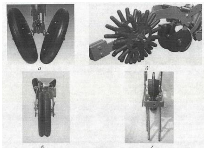
Fig. 9. Rolling mills: a - K-shaped roller; b - finger sealing roller; c - sealing roller; d - heavy roller with restrictive flanges.
