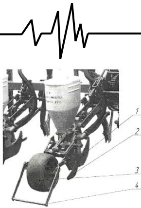
Fig. 7. Seeder section SUPN - 8A: 1 - opener; 2 - wrapper; 3 - copying and rolling roller; 4 - loop
