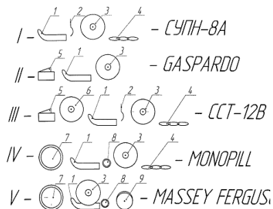
Fig. 2. Technological schemes of opener groups: I, II, III, IV, V - options: 1 - opener; 2 - wrapper; 3 - copying rolling roller; 4 - loop; 5 - lump separator; 6 - copying sealing roller; 7 - disk knife (coulter); 8 - suction wheel; 9 - V-shaped rolling roller.
