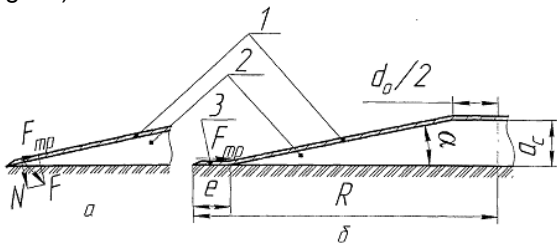
Fig. 12. The scheme of influence of soil on a blade of a plate opener: a - without a rim; b - with a rim; 1 - plate opener; 2 - space under the opener; 3 - horizontal lunch; e - rim width.
