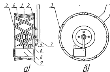
Fig. 4. Lump separator of the opener group of a row seeder: a - lump separator, front view; b - lump separator, side view; 1 - skating rink; 2 - right vertical disk; 3 - left vertical disk; 4 - rib; 5 - axis; 6 - bearing assembly; 7- bracket; 8 - rack plate blade; 9 - plate blade.
