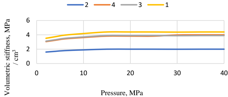
Fig. 1. Graphs of the dependence of the reduced volumetric stiffness coefficients on pressure: 1 – pressure dependence of the coefficient of reduced volumetric stiffness of a high pressure hose with a nominal diameter d_1 = 16 mm, the length of which, without taking into account the length of the fitting nipples (net length of the rubber-cord sheath), is L_{11} = 0.94 m; 2 – pressure dependence of the coefficient of reduced volumetric stiffness of the same high pressure hose, the length of which, without taking into account the length of the fitting nipples, is L_{12} = 1.94 m; 3, 4 – pressure dependences of the coefficients of the reduced volumetric stiffness of the same hoses, recalculated according to equation (5) per 1 meter of their length
