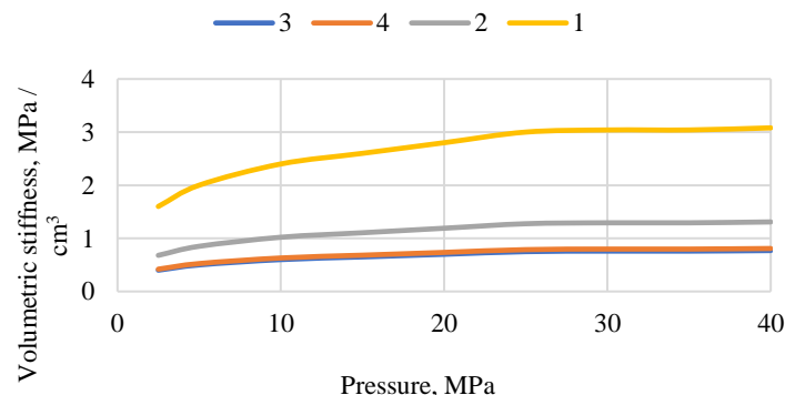
Fig.3. Graphs of the dependence of the coefficients of the reduced volumetric stiffness of the high pressure hose on pressure when they are included in the circuit in series: 1 - pressure dependence of the coefficient of reduced volumetric stiffness of high pressure hoses with a nominal diameter d_1 = 16 mm, the net length of the rubber-cord shell of which is L_{12} = 1.94 ; 2 - pressure dependence of the coefficient of the reduced volumetric stiffness of the high pressure hose with a nominal diameter d_2 = 32 mm, the net length of the rubber cord shell of which is L_{21} = 0.88 ; 3, 4 - pressure dependences of the coefficients reduced volumetric stiffness of the above sleeves connected in parallel in the circuit; (3 - determined by equation (5) using experimental data)
