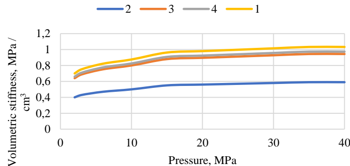
Fig.2. Graphs of the dependence of the coefficients of reduced volumetric stiffness on pressure: 1 – pressure dependence of the coefficient of reduced volumetric stiffness of a high pressure hose with a nominal diameter d_2 = 32 mm, the length of which, without taking into account the length of the fitting nipples, is L_{21} = 0.88 m; 2 – pressure dependence of the coefficient of reduced volumetric stiffness of the same high pressure hose, length which, without taking into account the length of the fitting nipples, is L_{22} = 1.88 m; 3, 4 – pressure dependences of the coefficients of the reduced volumetric stiffness of the same hoses, recalculated according to equation (5) per 1 linear meter of their length
