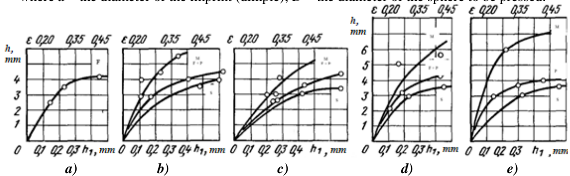
Fig. 8. Dependence of the depth of the riveted zone h from the depth of the print h_1 for carbon steels with different structures: a – iron; b – steel 35; c – steel 45; d – steel 60; e – U8; F – ferrite; M – martensite; P – pearlite; S – sorbite
