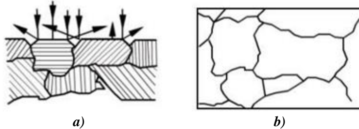
Fig. 2. Detecting the microstructure of an alloy: a – scheme of forming an image from the surface of an etched grind; b – etched sample with a homogeneous phase structure.
